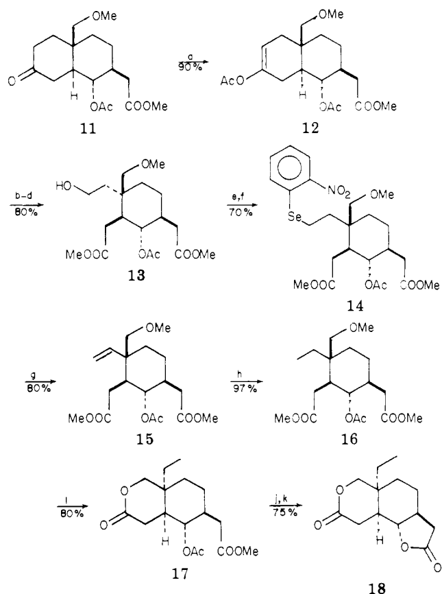
Scheme I. Synthesis of Bisnordihydrodeoxyvernolepin (18)
